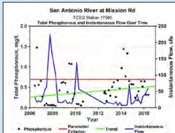
Fig. USAR 6: 17066 SAR at Mission Road, Total Phos over Time
