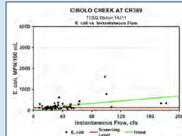
Fig. LCC 4: 14211 LCC at CR 389, E. coli against Flow
